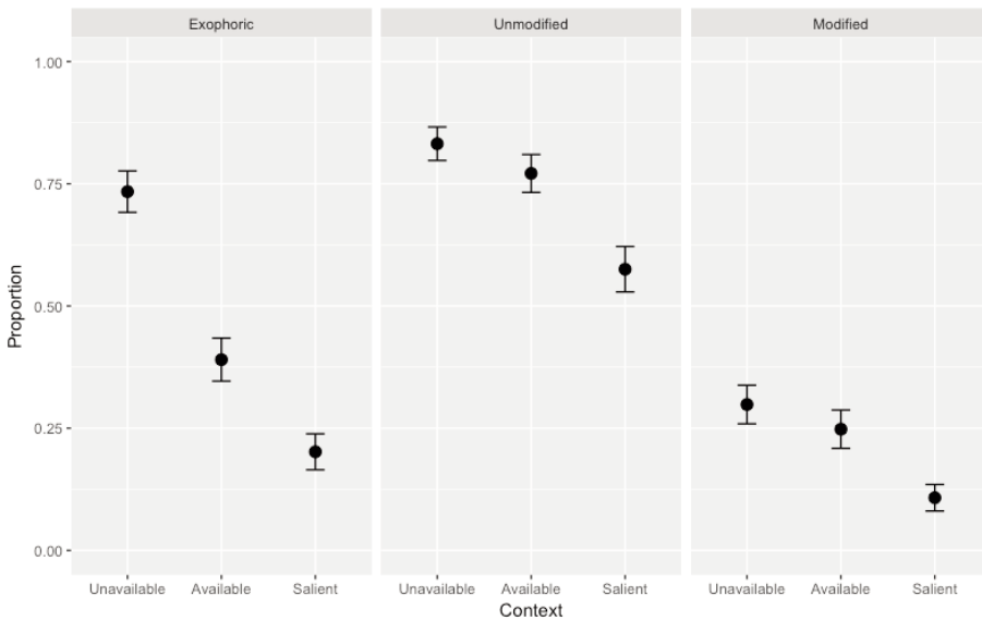
FIGURE 3. Experiment 1 results: proportions of polar responses. The error bars represent by-participant standard errors. 2
